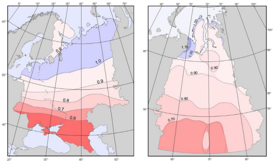
Figure 29 Relative changes (within the area of the East European Plain (left) and Western Siberia (right)) of the annual rivers runoff for the middle of the 21st century (reference volume is the values for current climate). Figures from Kasimov and Kislov, 2011.
