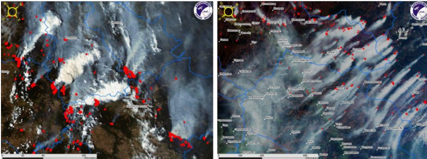
Figure 32 Fires in Central Russia (left) and Siberia and Urals (right). Satellite figures from Valery Bondur, AEROCOSMOS.
